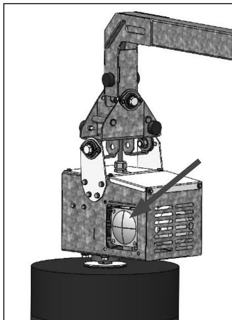
Figure 10: Mounting position of the sensor board
