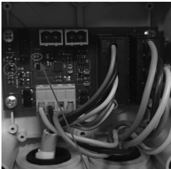
Illustration 11: Sensorprintkort
